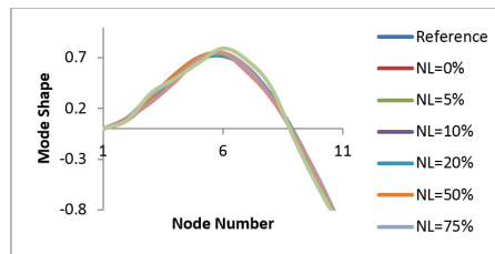
Figure 5: The second mode shape of beam CF
