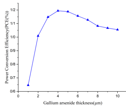
Fig. 7. Power conversion efficiency variation with GaAs substrate thickness.
