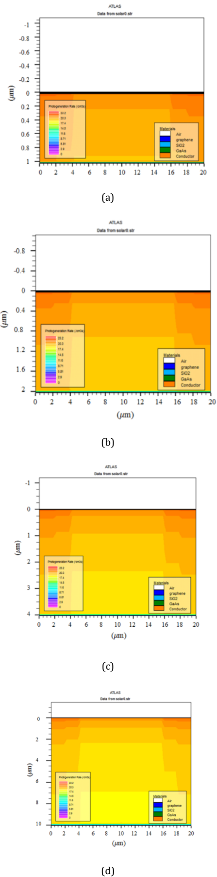
Fig. 3. Carrier generation rate in the graphene/GaAs solar cell under AM1.5 illumination standard for different substrate thicknesses: (a) 1 \mu\text{m} , (b) 2 \mu\text{m} , (c) 4 \mu\text{m} , and (d) 10 \mu\text{m} .
