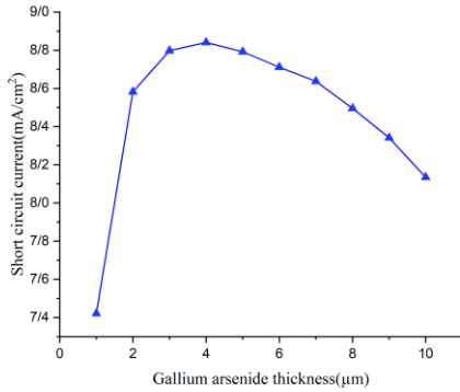
Fig. 4. Variation of short-circuit current density with GaAs substrate thickness.
