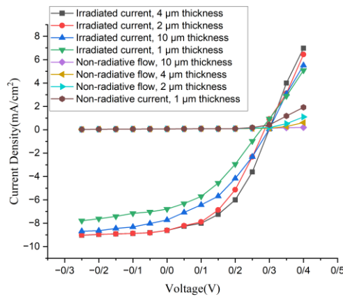
Fig. 2. Comparison of the current–voltage (I–V) characteristics of the graphene/GaAs solar cell for different GaAs substrate thicknesses.
