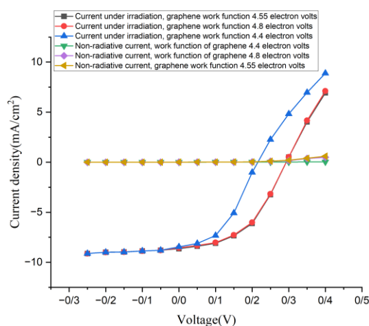
Fig. 8. Current-voltage (I-V) characteristics of the graphene/gallium arsenide solar cell considering three different graphene work function values.
