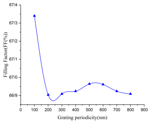
Fig. 11. Variation of fill factor with the periodicity of the rectangular nanograting.
