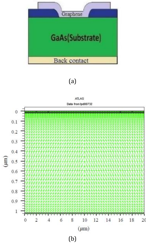
Fig. 1. (a) Cross-sectional view of the graphene/gallium arsenide (GaAs) Schottky-junction solar cell. (b) The designed mesh model of the structure.
