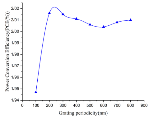
Fig. 12. Variation of power conversion efficiency with the periodicity of the rectangular nanograting.
