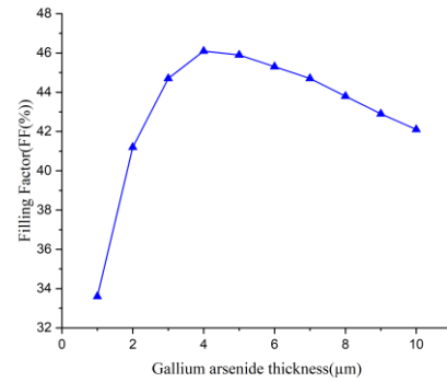
Fig. 6. Variation of fill factor with GaAs substrate thickness.
