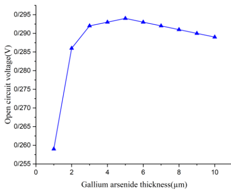
Fig. 5. Variation of open-circuit voltage with GaAs substrate thickness.
