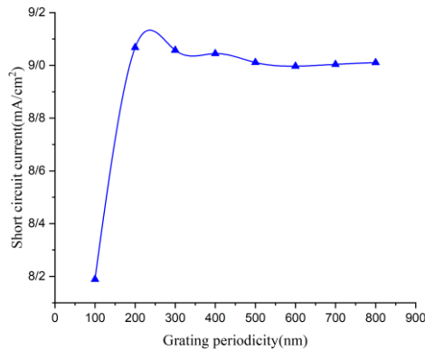
Fig. 10. Variation of short-circuit current with the periodicity of the rectangular nanograting.
