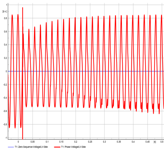
Fig. 13. LV side phase voltage with flux 1.3
