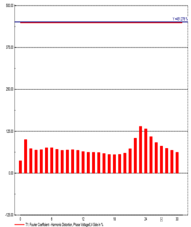
Fig. 20. LV side phase voltage harmonic distribution with flux 1.9
