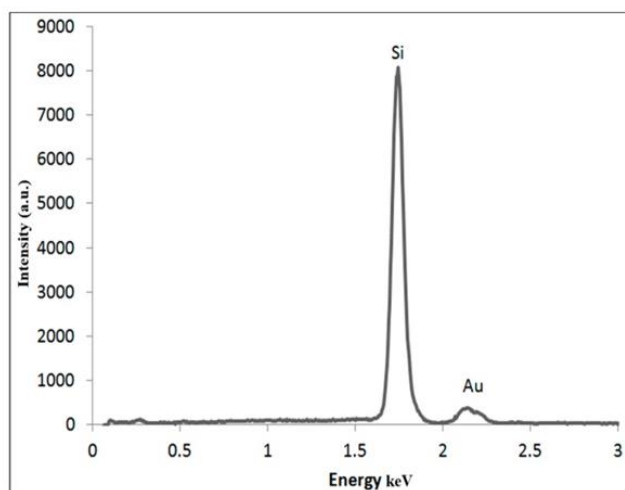
Fig. 8. EDX spectrum of Lc -GNPs extract.
