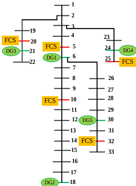
Fig. 3: IEEE 33-bus electrical network
