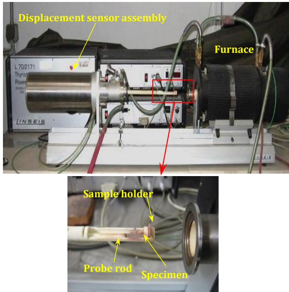
Figure 5. Horizontal dilatometer
