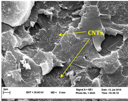
Figure 15. SEM images of the fracture surface of EP+0.25%AFMWCNTs
