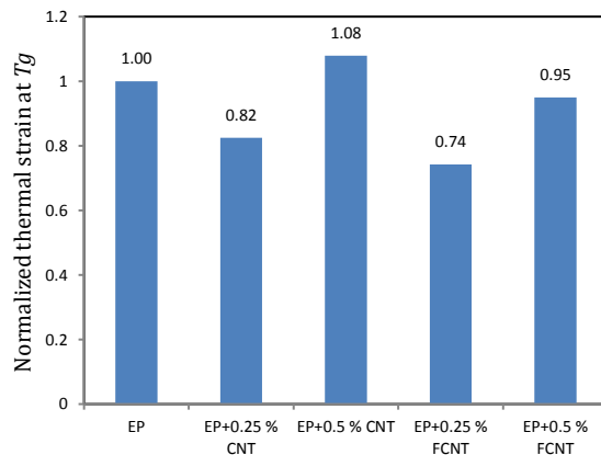
Figure 12. Normalized \epsilon_{T_g} of the nanocomposites
