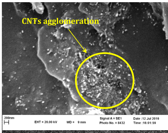
Figure 16. SEM images of the fracture surface of EP+0.5%AFMWCNTs
