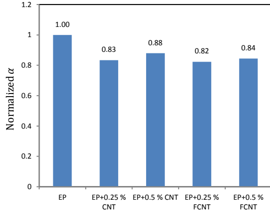
Figure 10. Normalized CTE of the nanocomposites
