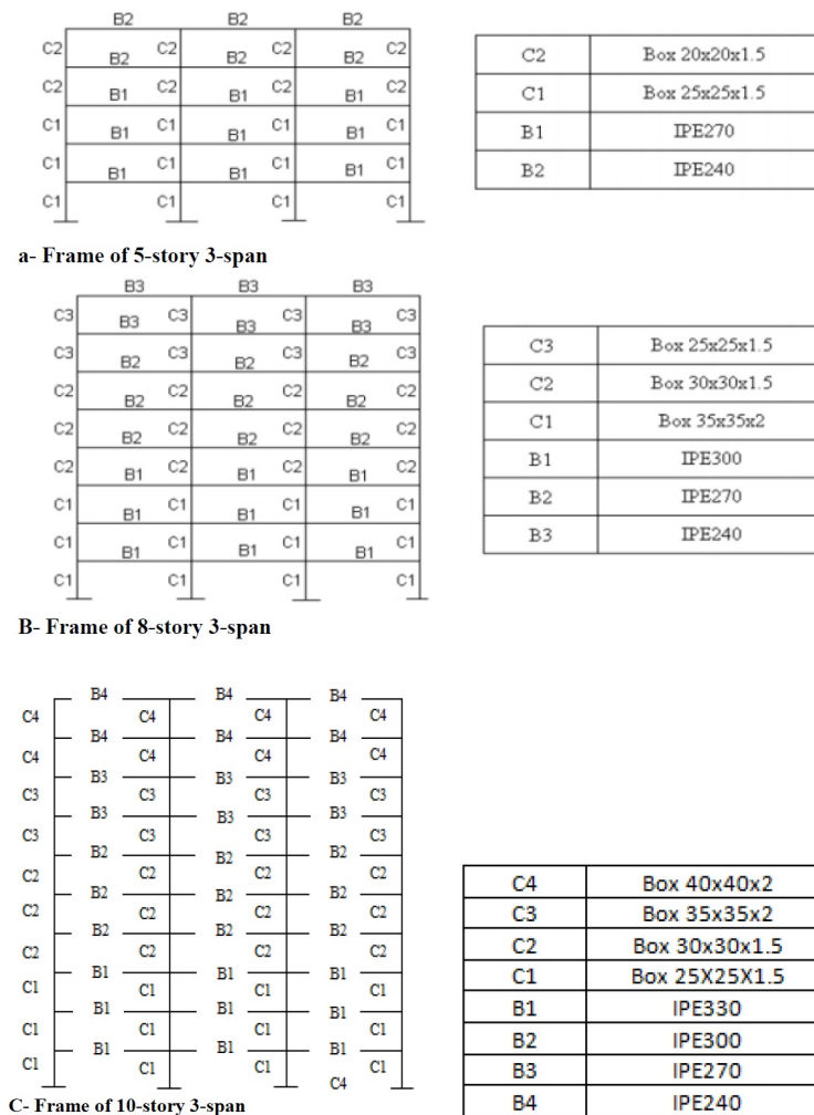
Figure 14: Modelling details
