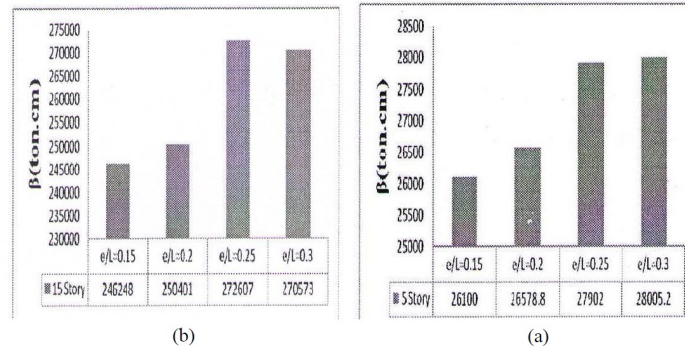
Figure 13: Behavior coefficient corresponding to different lengths. (a): five story frames, (b): fifteen story frames
