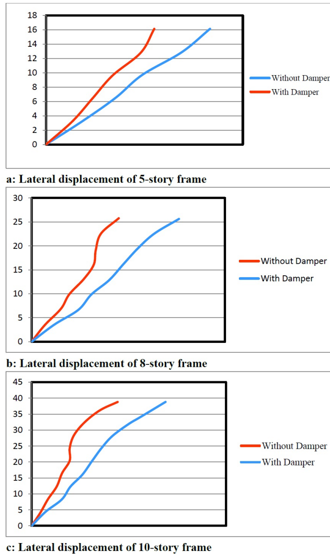
Figure 15: Lateral displacement of 5-story frame, 8-story frame and 10-story frame
