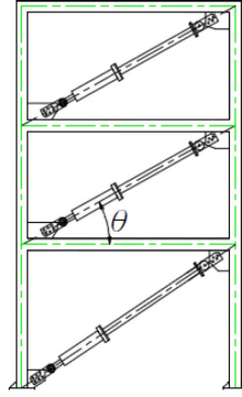
Figure 4: Multiple-degrees-of-freedom of a structure equipped with viscous dampers
