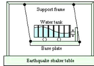
Figure 5: Damper tuned liquid
