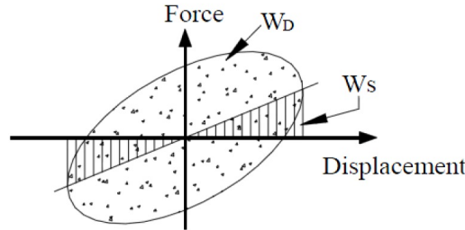
Figure 3: W_D absorbed energy in a harmonic movement cycle and maximum strain energy of a one-degree-of-freedom system or a damper
