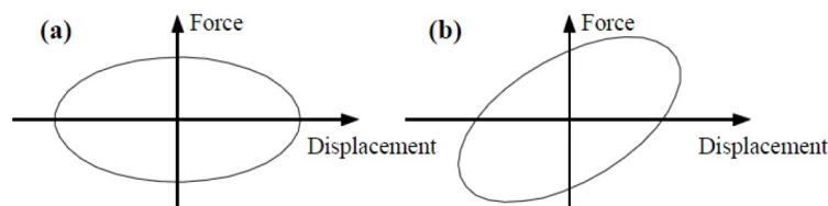
Figure 2: Hysteresis cycle of dampers with the behavior of linear and nonlinear viscous
