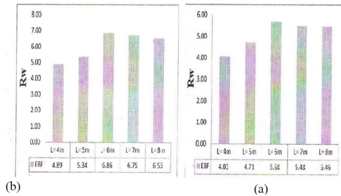
Figure 12: Behavior coefficient corresponding to different lengths. (a): five story frames, (b): fifteen story frames
