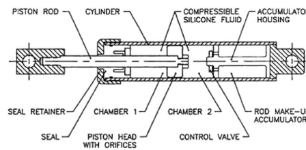
Figure 6: The structure of Fluid viscous damper
