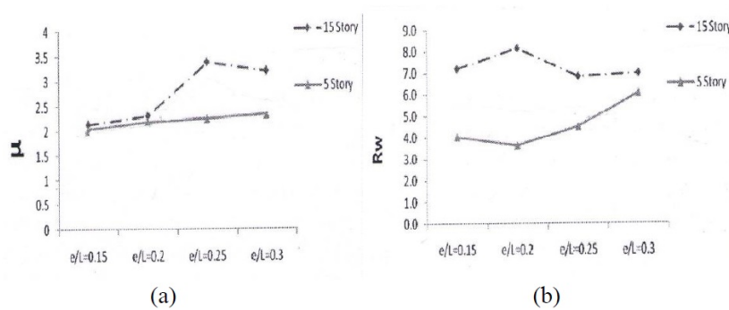
Figure 11: (a) Changing curve (b) Behavior coefficient. Plasticity for discussed frames
