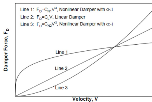
Figure 1: Force-velocity relations of viscous dampers
