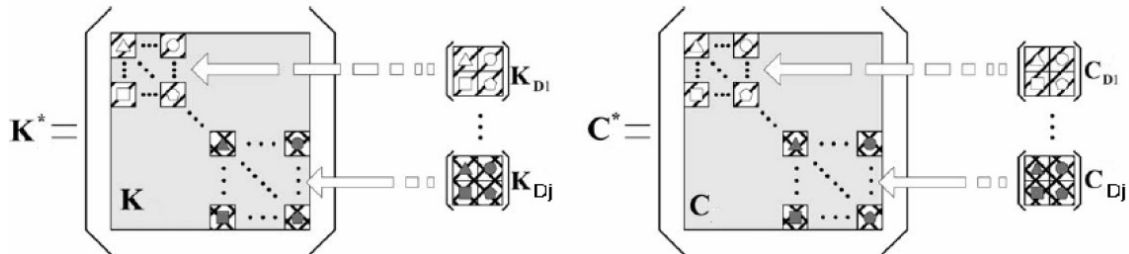
Figure 9: Adding damper's hardness and damping matrices to structure's hardness and damping matrices [8]
