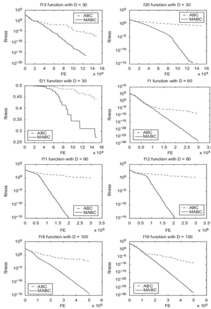
Figure 1: Different ABC convergence performance test functions
