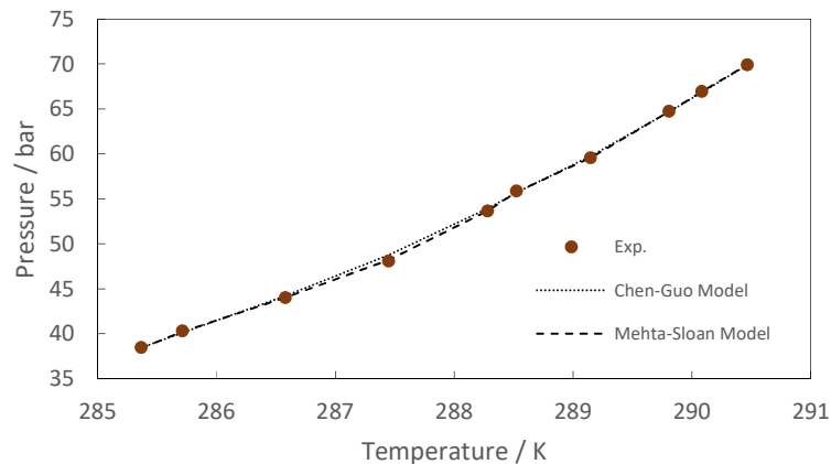
Figure 1. Correlated and experimental hydrate dissociation conditions in methane + 1-methylpiperidine + water system, experimental data (●) [13], (.....: Chen-Guo model [5] results), (----: Mehta-Sloan model [4] results)
