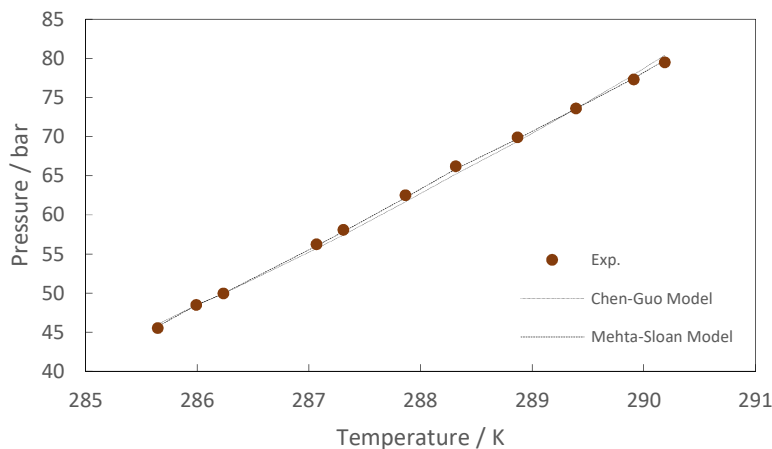
Figure 1. Correlated and experimental hydrate dissociation conditions in methane + 1-methylpiperidine + water system, experimental data (●) [13], (.....: Chen-Guo model [5] results), (----: Mehta-Sloan model [4] results)
