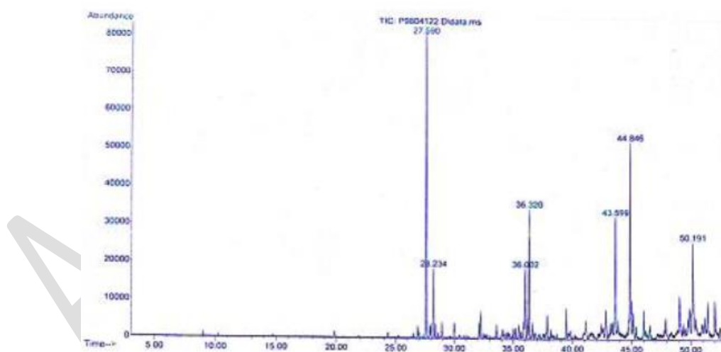
Figure 2. GC/MS analysis for subcritical water extraction for 2 g of grounded Fennel. (Mean particle size between 0.5 to 0.71 mm, temperature 125 ^{\circ}\text{C} , flow rate 1.25 ml/min, extraction time 65 min).
