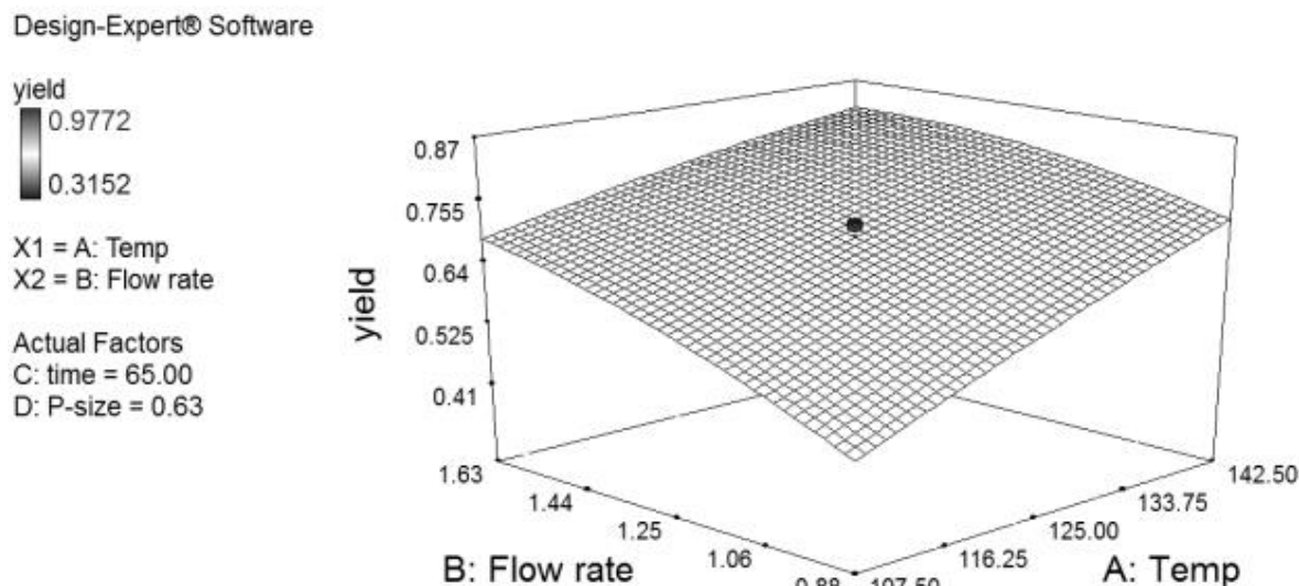
Figure 3. The extraction yield versus the simultaneous effect of temperature (A) and flow rate (B).
