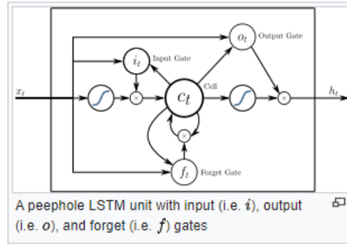
Figure 5: LSTM network
