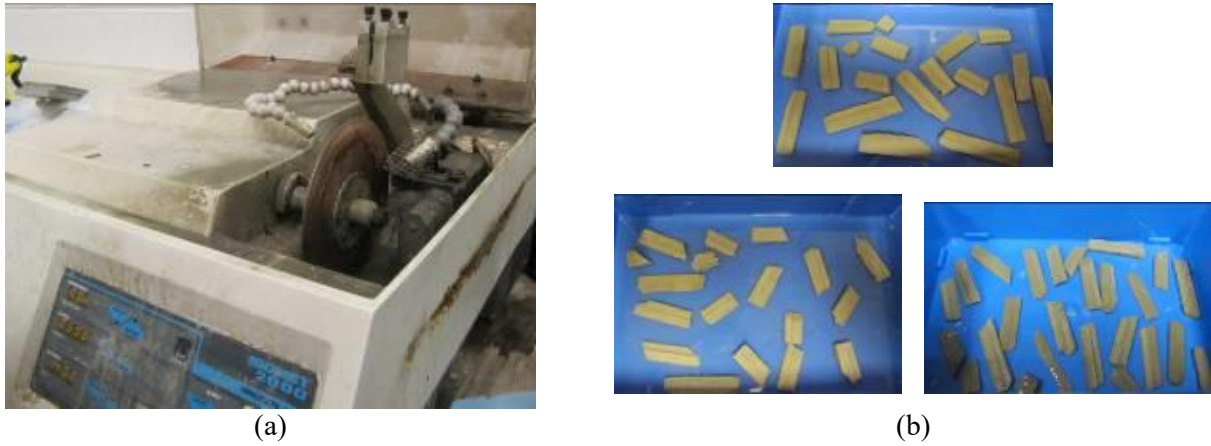
Fig. 6. High precision saw (a) and single fiber specimens cut ready for testing (b).
