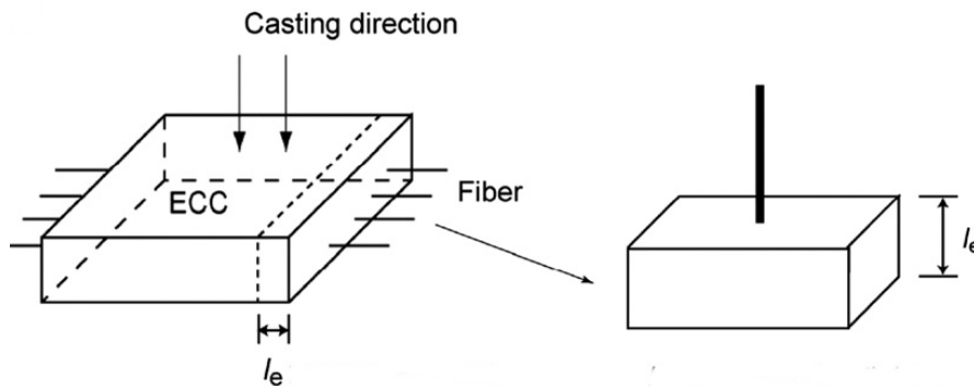
Fig. 7. Final specimen shape - l_e : embedded fiber length [23].
