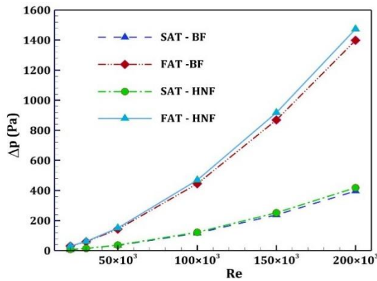
Fig. 13. Variation of the pressure drop with Re for the SAT and the IFAT
