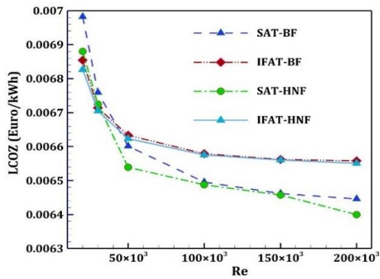
Fig. 20. The LCOE of the PTC with the Re for the finned and smooth absorber tubes
