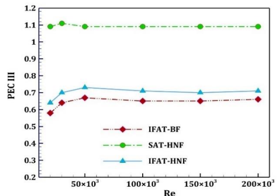
Fig. 17. Variation of the PEC III of the PTC with the Re
