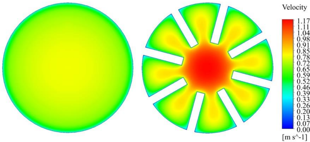
Fig. 8. Fluid outlet velocity contours in the SAT and the IFAT for the BF at Re=2 \times 10^5
