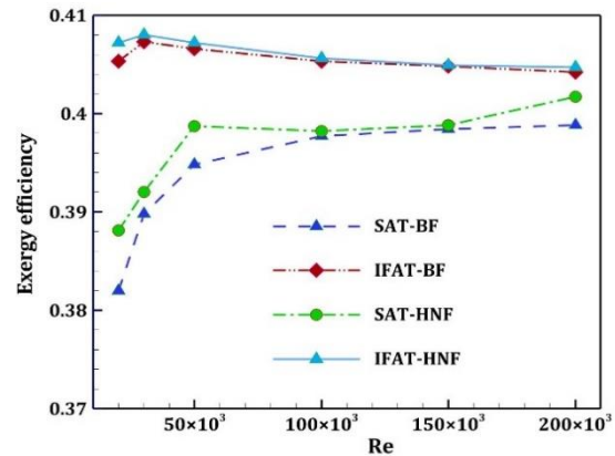
Fig. 19. Variation of the exergy efficiency of the collector for the SAT and the IFAT
