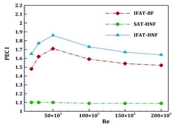
Fig. 15. Variation of the PEC I of the PTC with the Re
