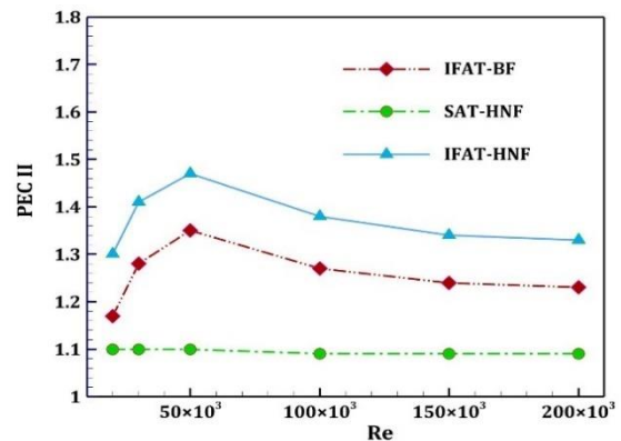
Fig. 16. Variation of the PEC II of the PTC with the Re
