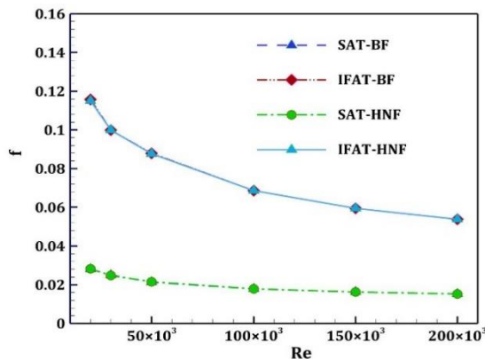
Fig. 14. Variations of the friction factor with the Re for the SAT and the IFAT
