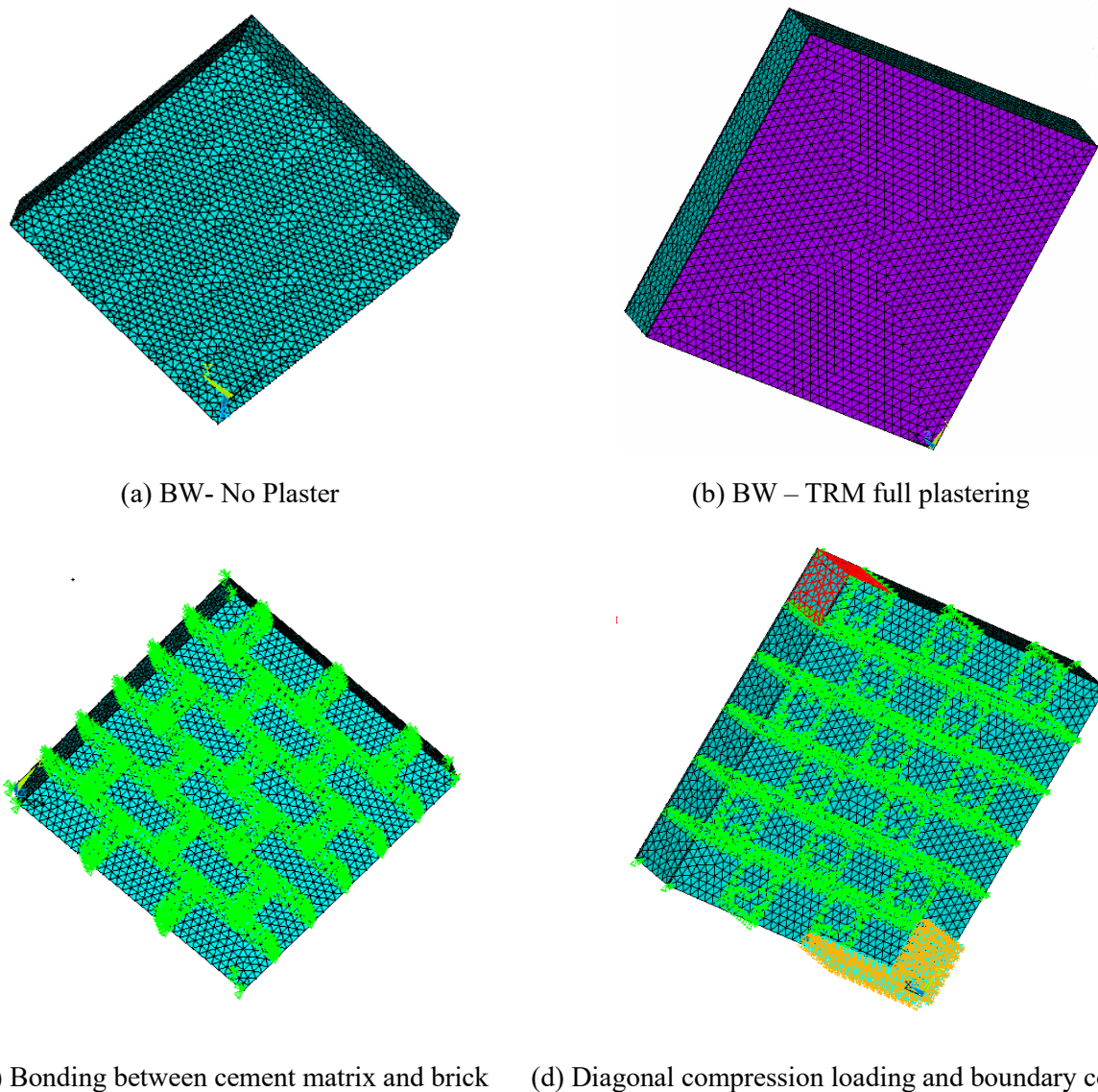
Fig. 6. Mesh mode, loading and boundary condition of Brick Masonry wallets.
