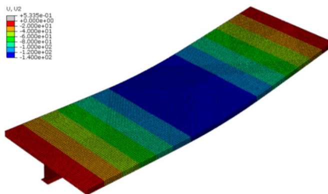
Fig. 9. Displacement of the developed FE model in Y direction.
