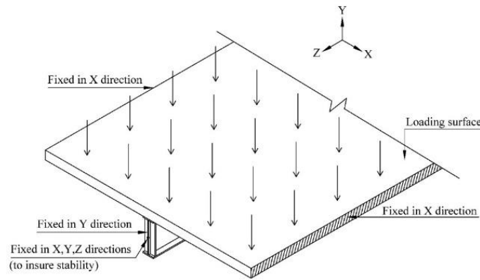
Fig. 4. Boundary conditions of the model.
