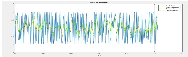
Figure 1: Estimation of the function by the method Linear, Hard Thresholding and Block Thresholding
