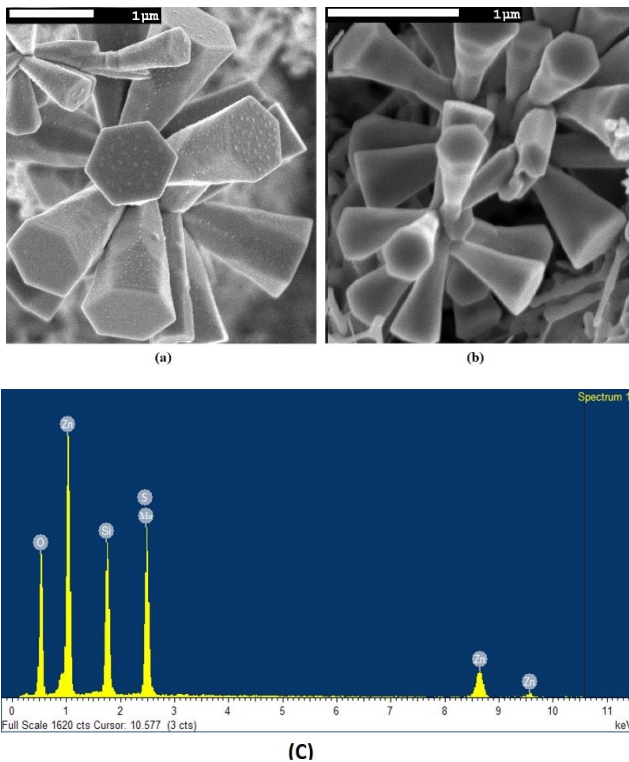
Fig. 3. FESEM images of (a) pure ZnO, (b) MoS 2 /ZnO, and (c) EDX image of MoS 2 /ZnO thin films
