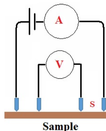
Fig. 1. Four- point- probe method
