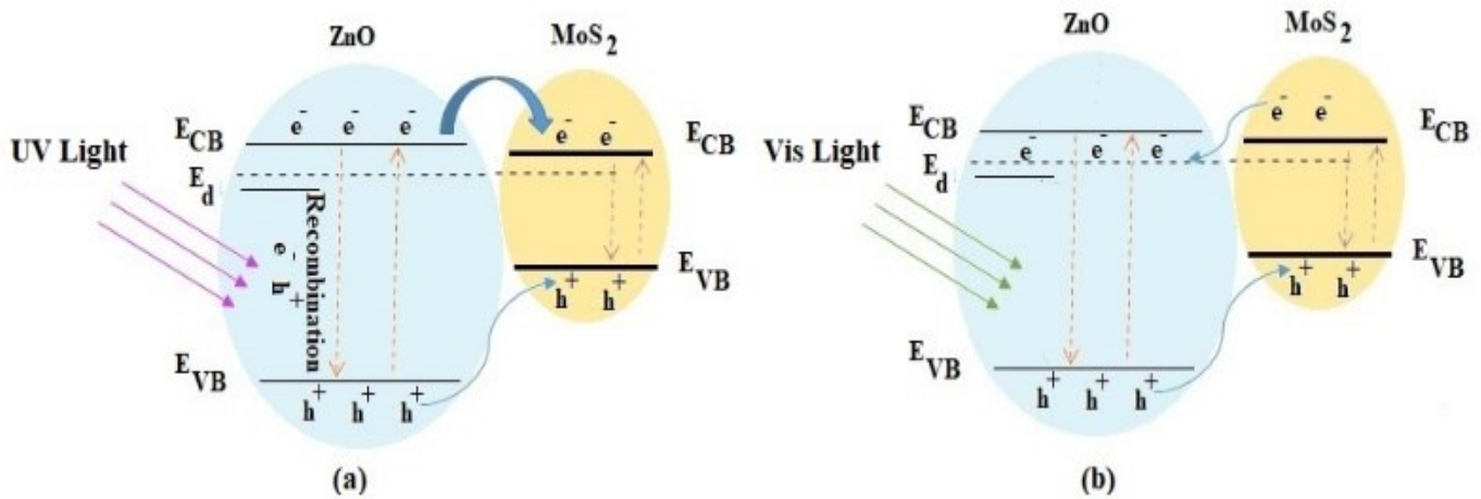
Fig. 8. Schematic illustration of the charge transfer process and energy level diagrams of pure ZnO and MoS 2 /ZnO thin film
