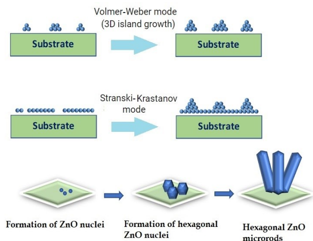
Fig. 10. Schematic illustration of two kinds of thin film growth modes and the possible growth mechanism for the formation of hexagonal microrods
