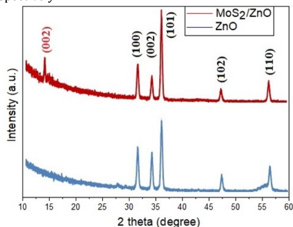
Fig. 2. XRD patterns of pure ZnO and MoS 2 /ZnO thin films
