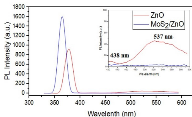
Fig. 7. PL emission spectra of pure ZnO and MoS 2 /ZnO thin films under 325 nm excitation
