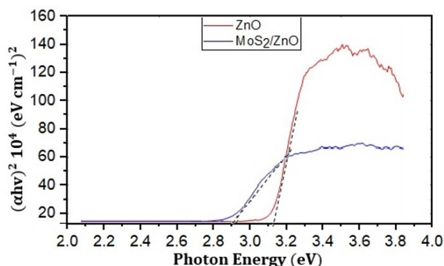
Fig. 6. Plots of the direct bandgap of pure ZnO and MoS 2 /ZnO thin films
