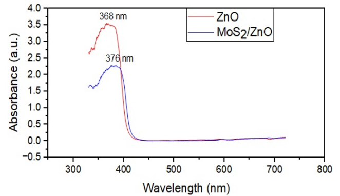
Fig. 5. The UV-Vis absorption spectra of pure ZnO and MoS 2 /ZnO thin films
