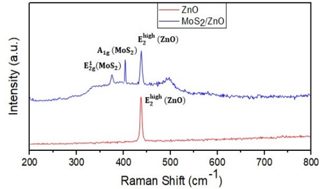
Fig. 4. Raman spectra of pure ZnO and MoS 2 /ZnO thin films
