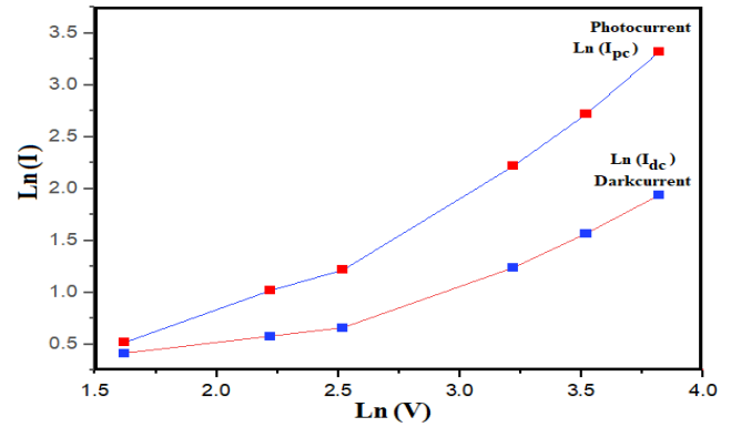
Fig. 9. Variation of photoelectric current ( I ) versus applied voltage for MoS 2 /ZnO thin film
