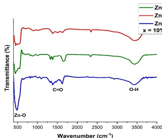
Fig. 3. FTIR spectra of ZnO prepared samples
