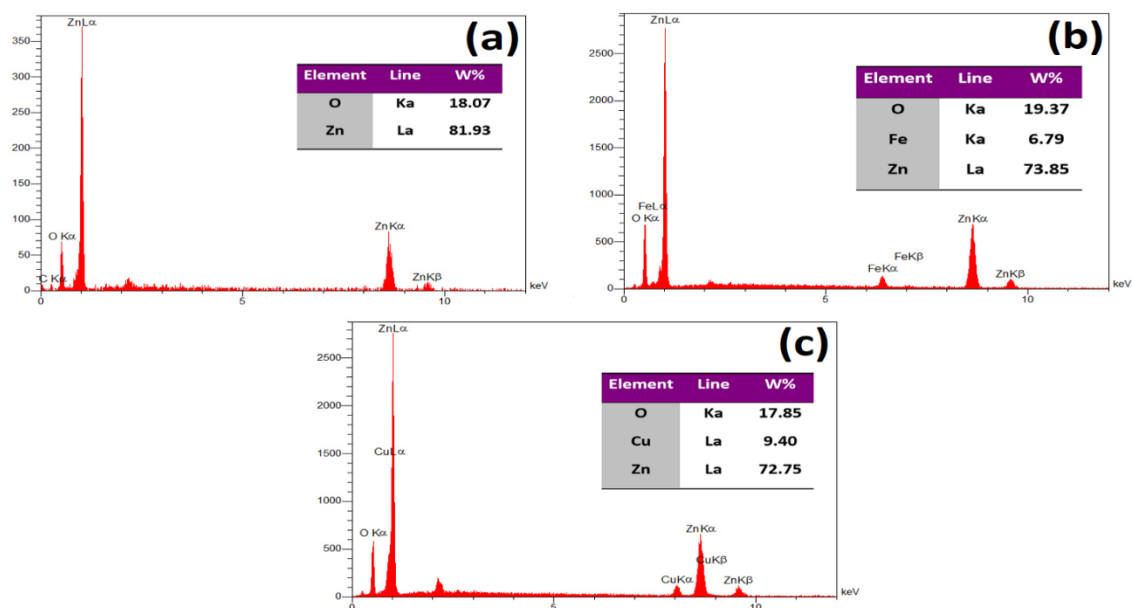
Fig. 5. EDS of the (a) ZnO, (b) \text{Zn}_{1-x}\text{Fe}_x\text{O} , and (c) \text{Zn}_{1-x}\text{Cu}_x\text{O} NPs
