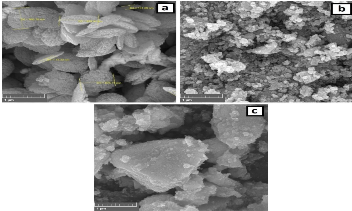
Fig. 4. FESEM images of (a) ZnO, (b) \text{Zn}_{1-x}\text{Fe}_x\text{O} and (c) \text{Zn}_{1-x}\text{Cu}_x\text{O} NPs
