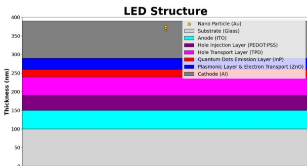
Fig. 2 . LED structure
