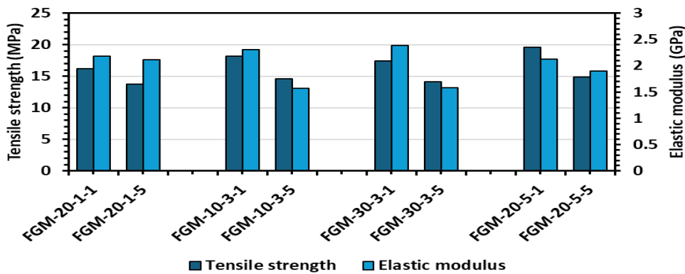
Fig. 10. The effect of masterbatch on tensile strength and elastic modulus at fixed percentages of DPF and PP-g-MA
