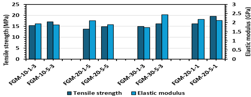
Fig. 9. The effect of PP-g-MA on tensile strength and elastic modulus at fixed percentages of DPF and masterbatch
