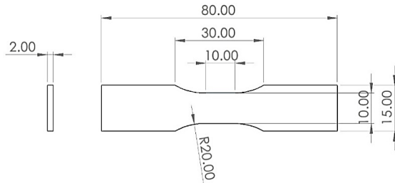
Fig. 2. The geometry of the tensile test specimen.
