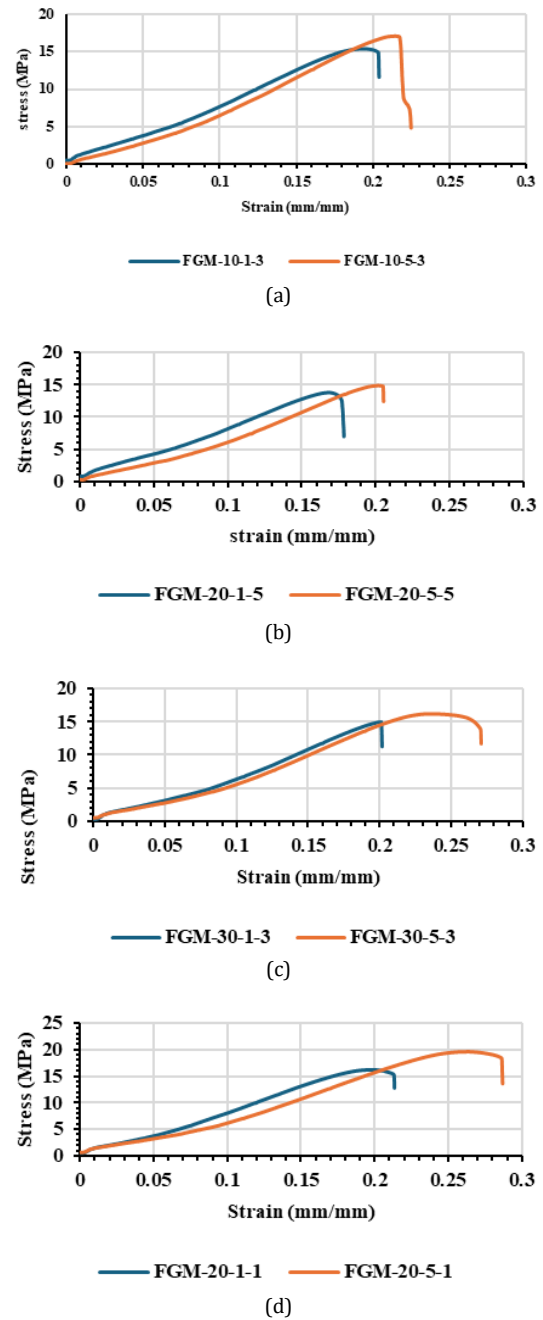
Fig. 13. Stress-strain diagrams of polypropylene/DPF composites at different PP-g-MA percentages
