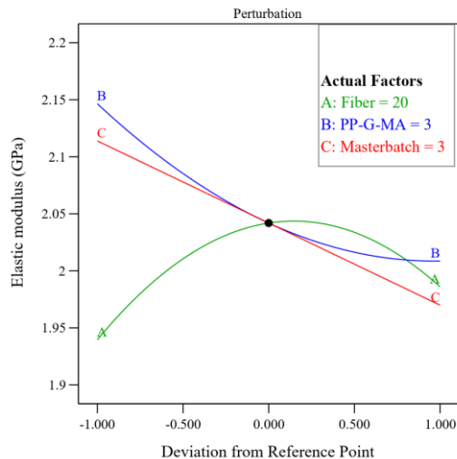
Fig. 14. Sensitivity analysis of parameters on the tensile modulus.
