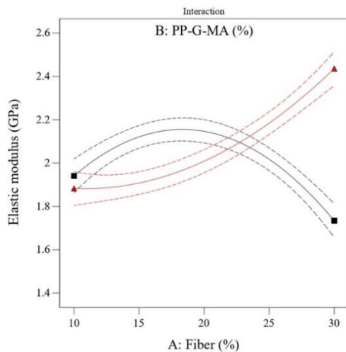
Fig. 15. Interaction between fiber percentage and compatibilizer on the elastic modulus response.
