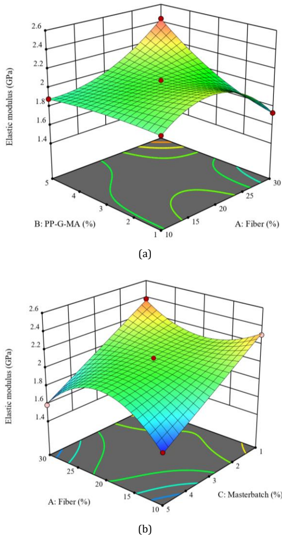
Fig. 12. a) Effect of DPF and PP-G-MA on the elastic modulus, b) Effect of DPF and masterbatch on the elastic modulus
