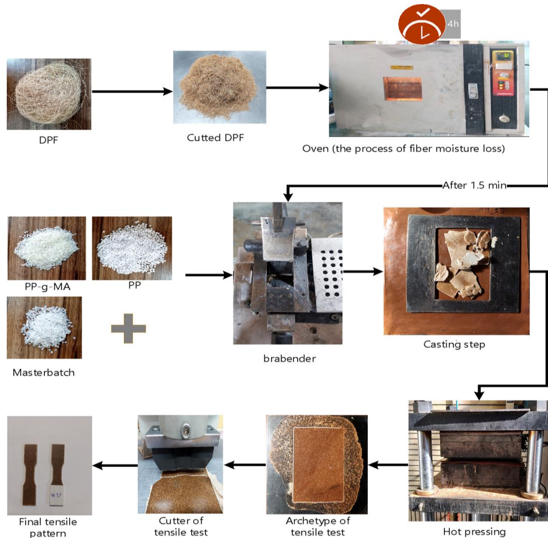
Fig. 1. The series of composite manufacture
