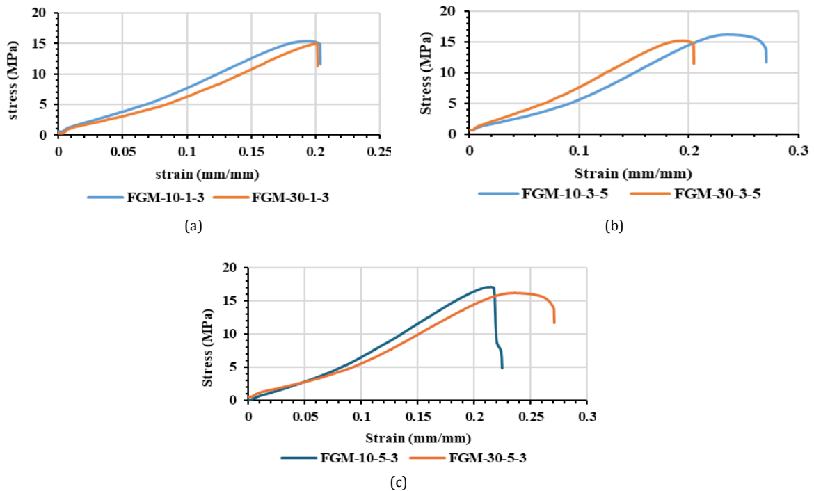
Fig. 7. Stress-strain diagram of polypropylene/DPF composite in different fiber percentages
