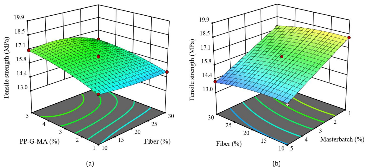
Fig. 8. (a) Effect of weight percentage of date palm fibers and PP-G-MA on tensile strength, (b) Effect of weight percentage of date palm fibers and masterbatch on tensile strength
