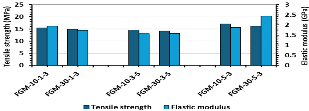
Fig. 6. The effect of DPF on tensile strength and elastic modulus in fixed percentages of PP-g-MA and Masterbatch
