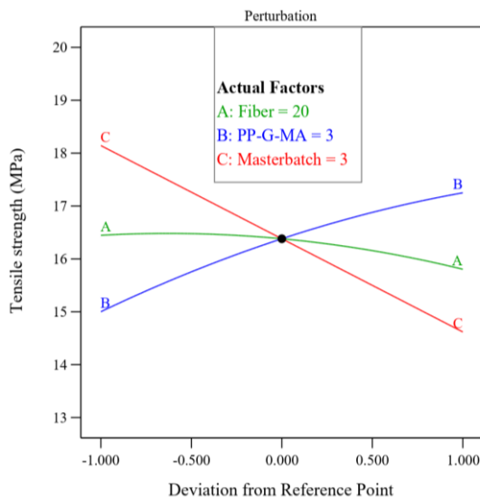
Fig. 11. Sensitivity analysis of parameters on the tensile strength
