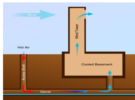
Figure 4: Diagram of a Qanat with Wind Tower [1]
