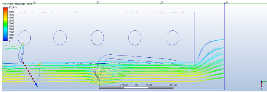
Diagram 1. Shell performance against flood flow (Source: Authors)
