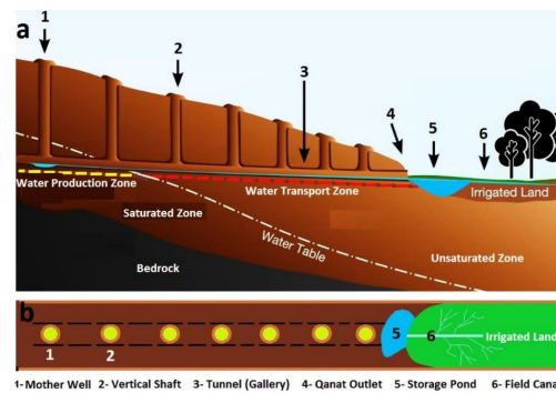
Figure 3: Schematic of a Qanat System: This figure illustrates a typical qanat system with two key perspectives: (a) a cross-section revealing the underground structure and (b) an aerial view showcasing the surface layout [17]
