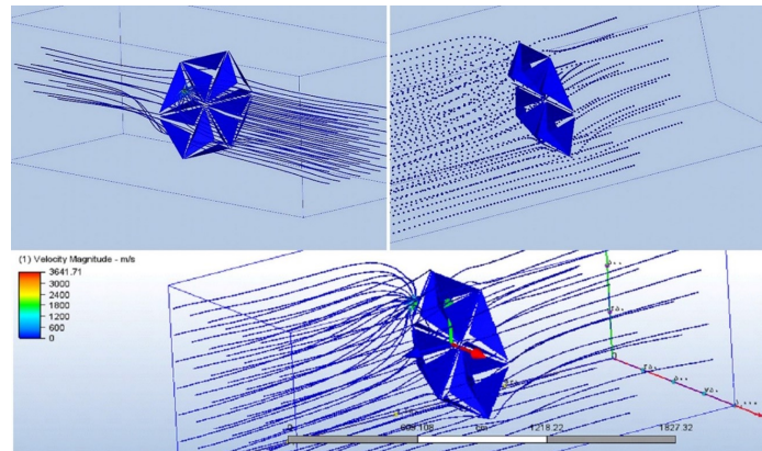
Figure 13: Images of the behavior of the shell against the flood flow in the software environment (Source: Authors)
