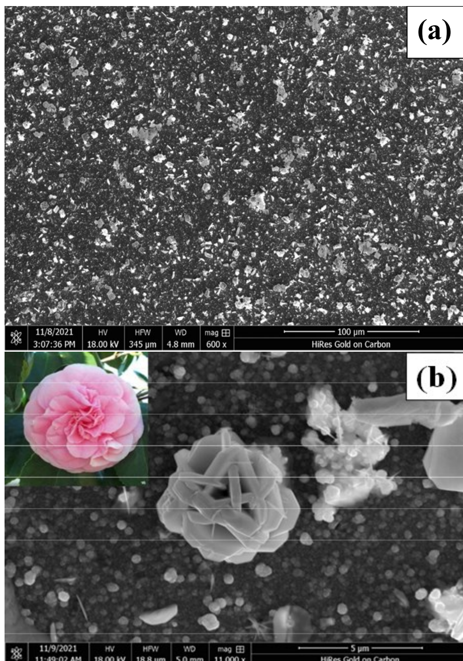
Fig. 6. FESEM micrographs of flower-like PbS nanostructure prepared by CBD deposited at 40 min (a) Low resolution images, (b) isolated PbS flower (Inset shows photographs of natural camellia flower)
