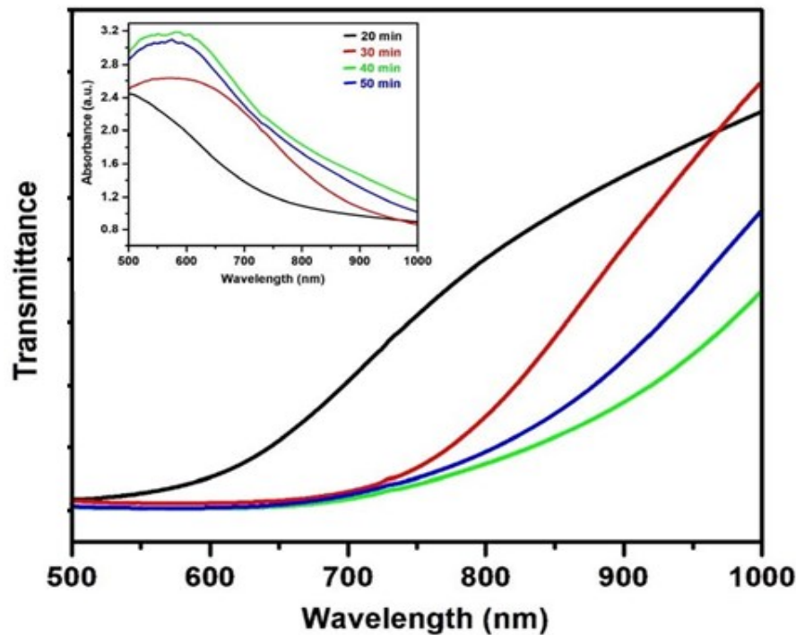
Fig. 9. Transmittance of nanocrystalline PbS thin films deposited on glass substrate at different deposition times. The inset shows the absorbance spectra obtained for the same thin films.
