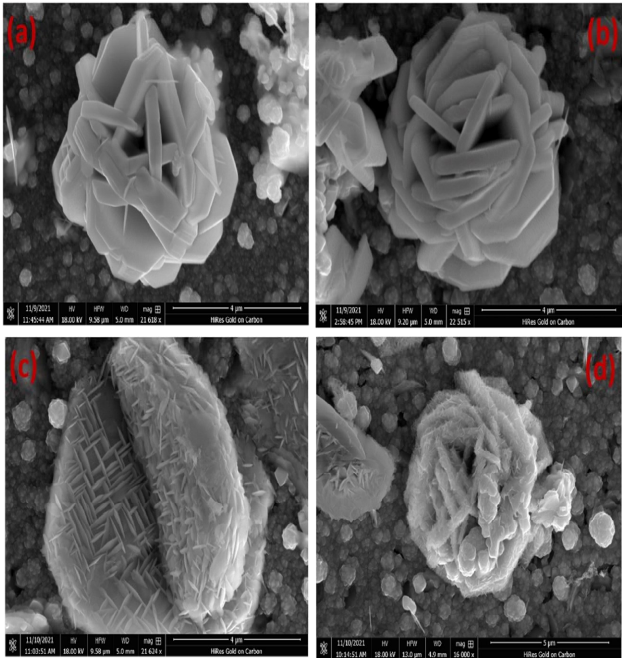
Fig. 7. The SEM images of PbS thin films representing flower like structures for different deposition times (a) 20 min, (b) 30 min, (c) 40 min, and (d) 50 min
