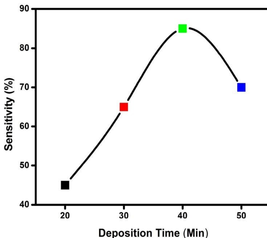
Fig. 13. Plot of PbS thin films deposition time against the sensitivity
