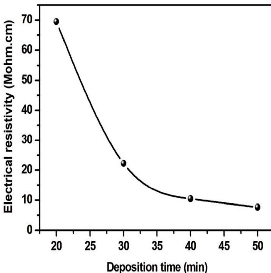
Fig. 12. Electrical resistivity versus deposition time of nanocrystalline PbS thin films
