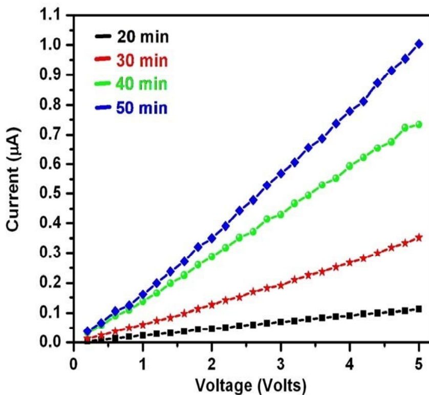
Fig. 11. Current voltage (I-V) characteristics of nanocrystalline PbS thin films prepared at different deposition time 20, 30, 40, and 50 min
