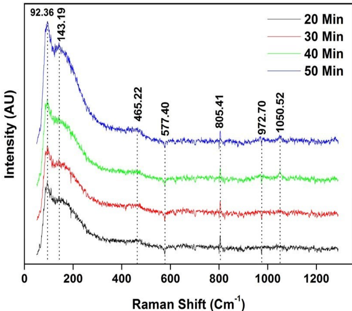
Fig. 4. Raman spectra for nanocrystalline PbS thin films deposited at time intervals of 20, 30, 40, and 50 min
