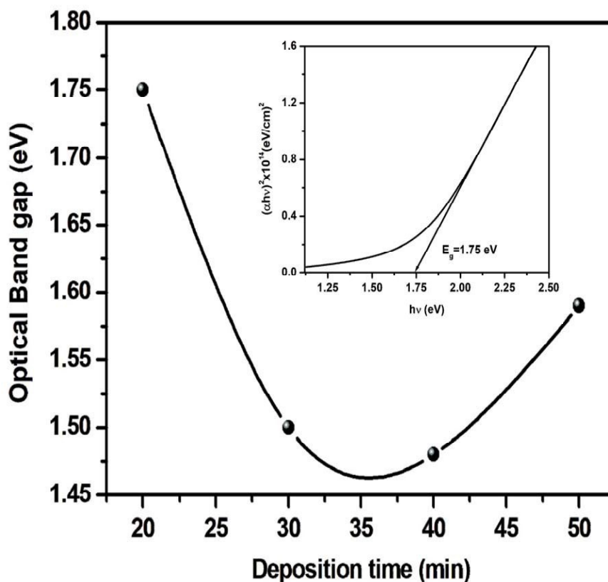
Fig. 10. Optical band gap versus deposition time of PbS thin films. The inset shows plot of (\alpha h\nu)^2 with respect to h\nu (eV) for nanocrystalline PbS thin films deposited in 20 min.
