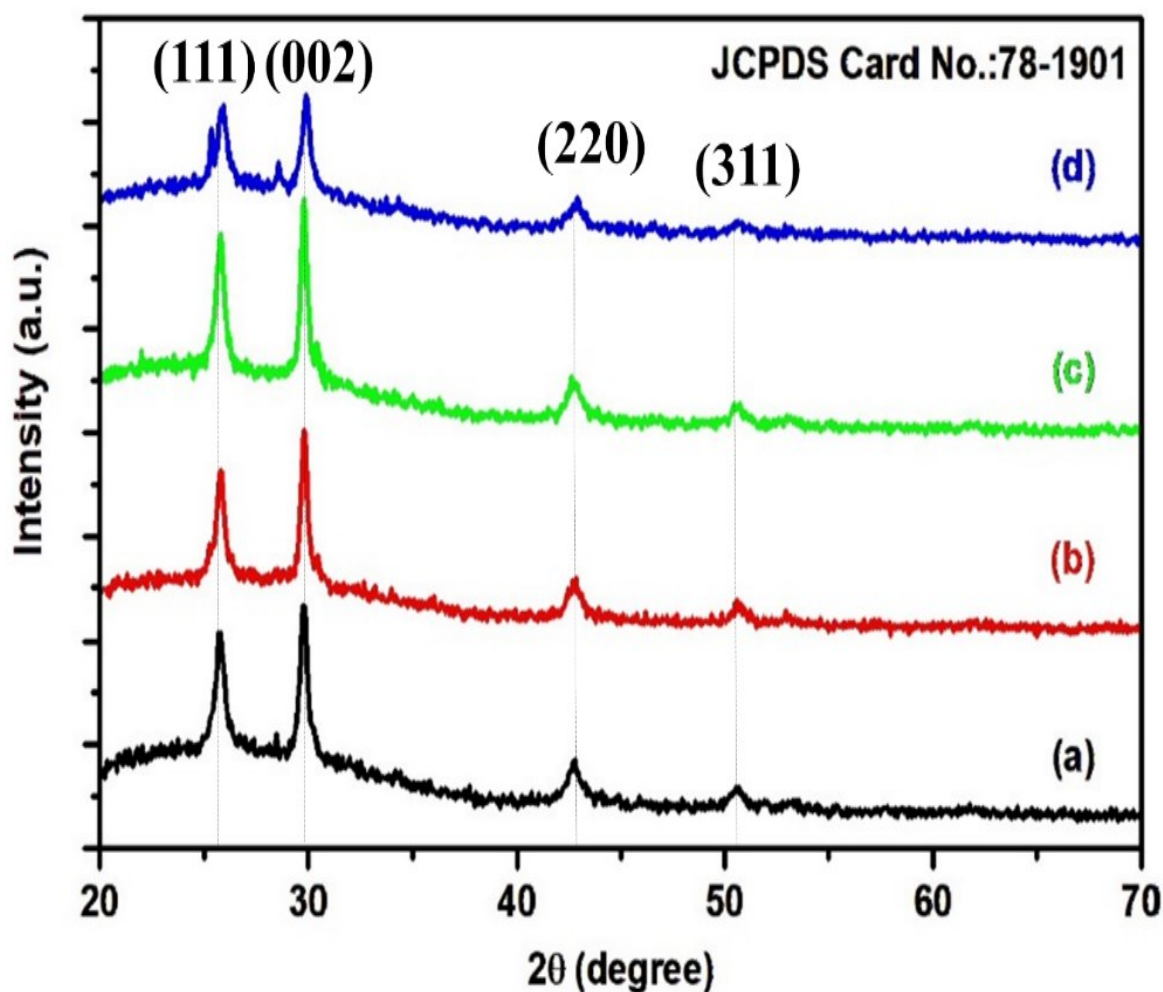
Fig. 3. X-ray diffraction (XRD) pattern of PbS thin film for different synthesis time represented by (a) 20 min, (b) 30 min, (c) 40 min, and (d) 50 min
