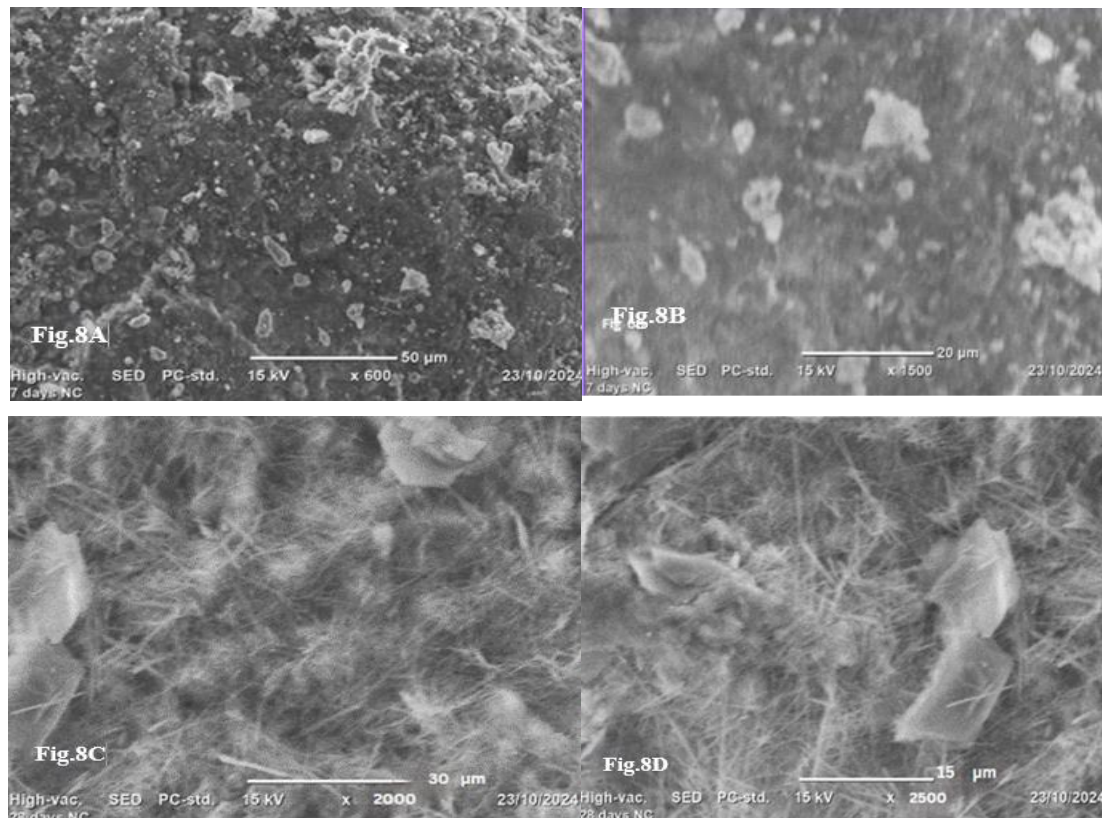
Fig. 8. Control concrete specimens that did not contain any incorporated healing agent showed cracks after 7 days of curing, as observed at 600 \times magnification (panel A) and 1500 \times magnification (panel B). Additionally, concrete specimens that did not contain any incorporated healing agent exhibited cracks after 28 days of curing, as observed at 2000 \times magnification (panel C) and 2500 \times (panel D).
