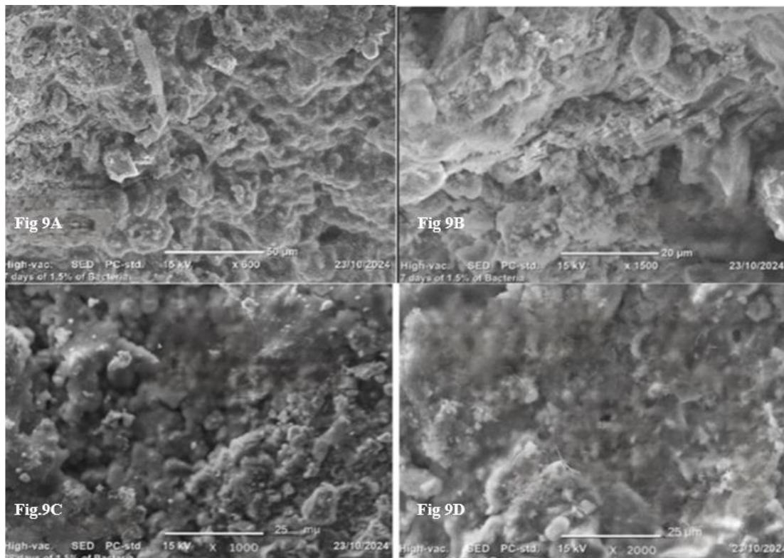
Fig.9. Shows concrete specimens with a healing agent were cracked after 7 days of curing (panels A: 600 \times and B: 1500 \times magnification) and 28 days of curing (panels C: 1000 \times and D: 2000 \times magnification). In specimens A and B, relatively large mineral precipitates, sized 18–78 \mu\text{m} , are visible. In contrast, those in specimens C and D are observed to be 5–8 \mu\text{m} in size.
