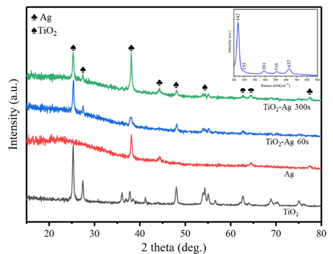
Fig. 2. XRD of \text{TiO}_2 , Ag, and Ag- \text{TiO}_2 films at 60s and 300s, showing anatase \text{TiO}_2 and FCC Ag. (Inset: Raman confirming anatase \text{TiO}_2 )
