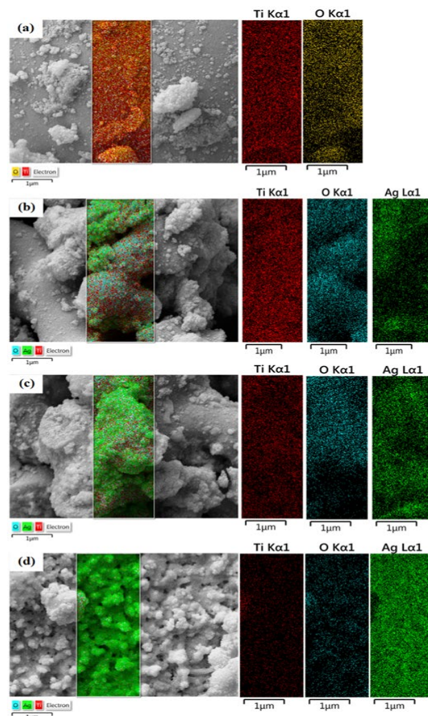
Fig. 4. EDX elemental mapping of (a) TiO 2 and Ag-TiO 2 films at deposition times of (b) 30s, (c) 60s, and (d) 300s
