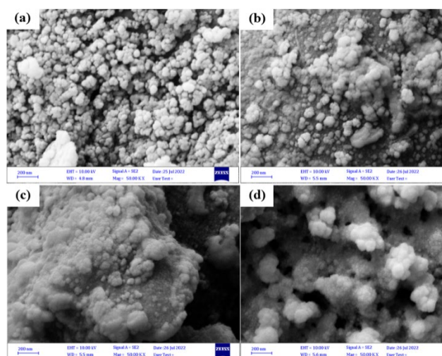
Fig. 3. FESEM images of (a) TiO 2 and Ag-TiO 2 films at deposition times of (b) 30s, (c) 60s, and (d) 300s
