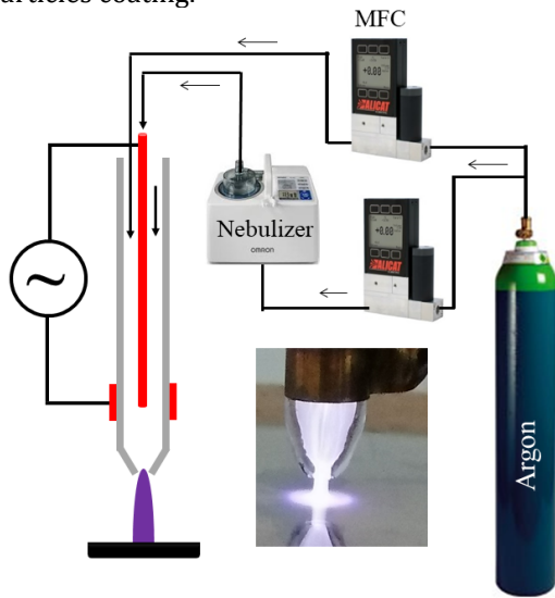
Fig. 1. Schematic and photograph of the plasma jet printing
