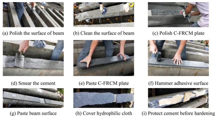
Fig. 8. Process of strengthening with prefabricated C-FRCM plate. Reproduced with permission from Feng et al. (2022)[23].
