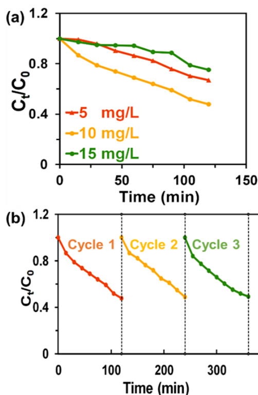
Fig. 6. (a) The effect of tetracycline concentration on photodegradation efficiency and (b) stability of the T(600) sample.
