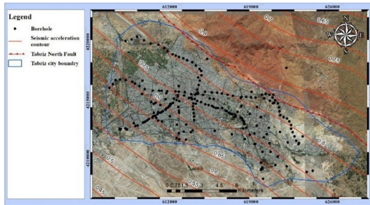
Figure 8: Distribution of PGA values in the study area based on the influence of soil layer magnification.
