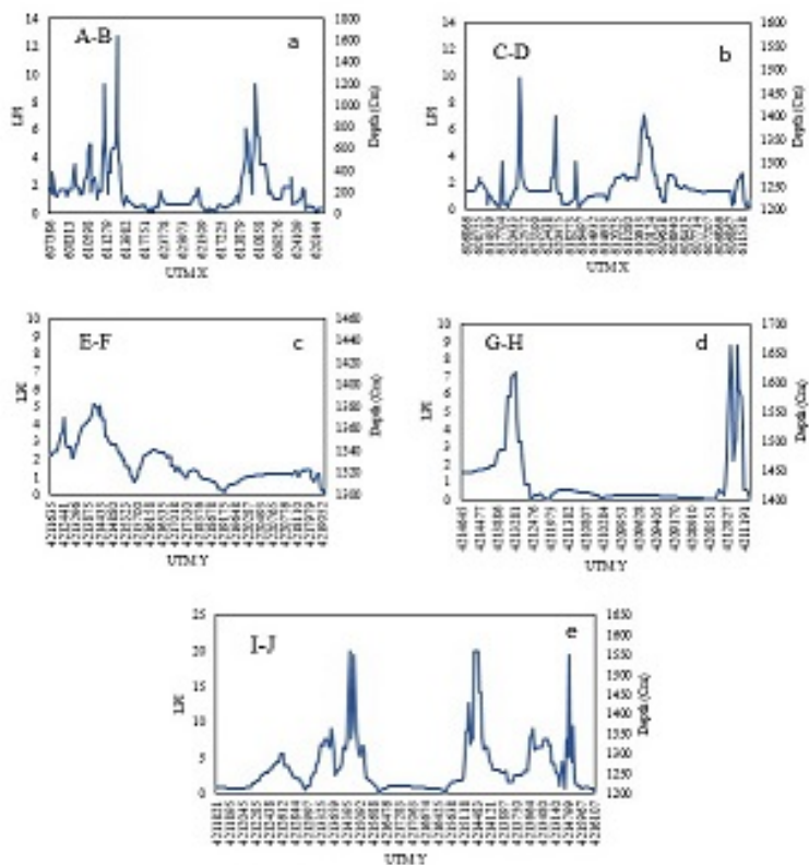
Figure 13: Variation of LPI in soil stratifications, a: A-B axes, b: C-D axes, c: E-F axes, d: G-H axes, e: I-J axes.
