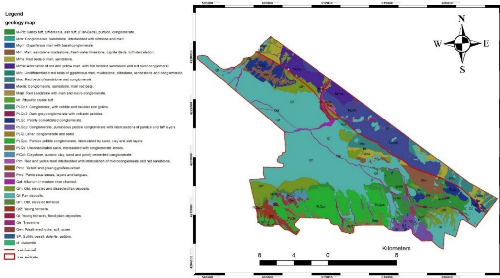
Figure 1: Geological Map of Tabriz.
