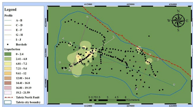
Figure 12: Location of five axes in study area for evaluation of LPI in soil layers.
