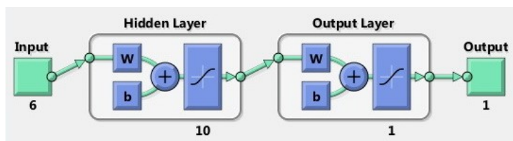
Figure 14: The frame of neural network analysis used in the present study.
