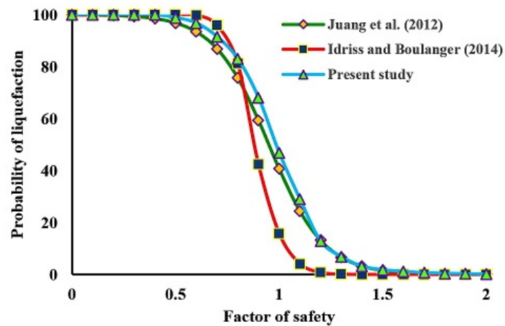
Figure 19: Comparison of diagram of liquefaction probability (in this study) with other methods based on safety factor parameter.
