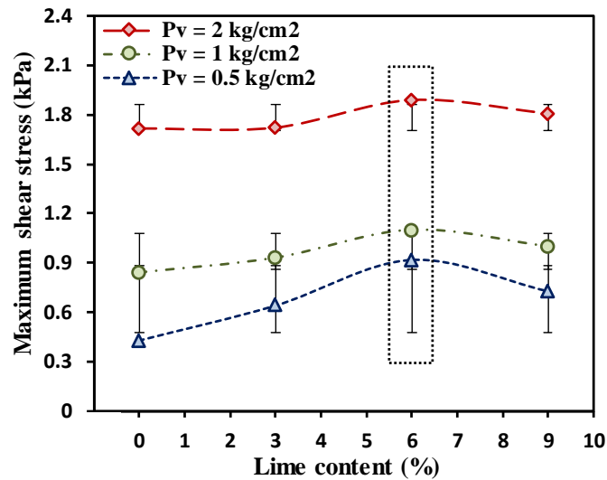
Fig. 7. The effect of lime-stabilization on the maximum shear strength of tested samples.
