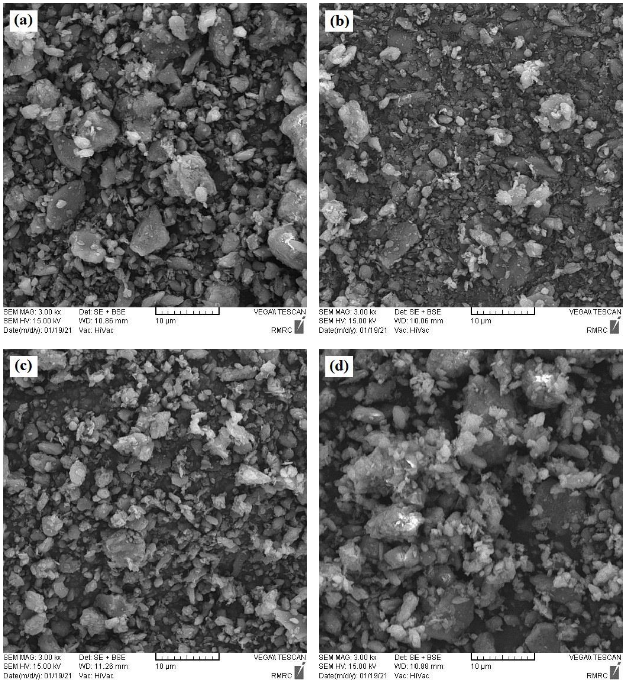
Fig. 10. SEM images with 10 \mu\text{m} scale, a) Landfill material, b) stabilized with 3 % lime, c) stabilized with 6 % lime, d) stabilized with 9 % lime.
