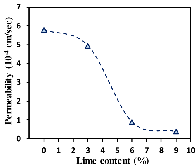
Fig. 8. The effect of lime-stabilization on the permeability of tested samples.
