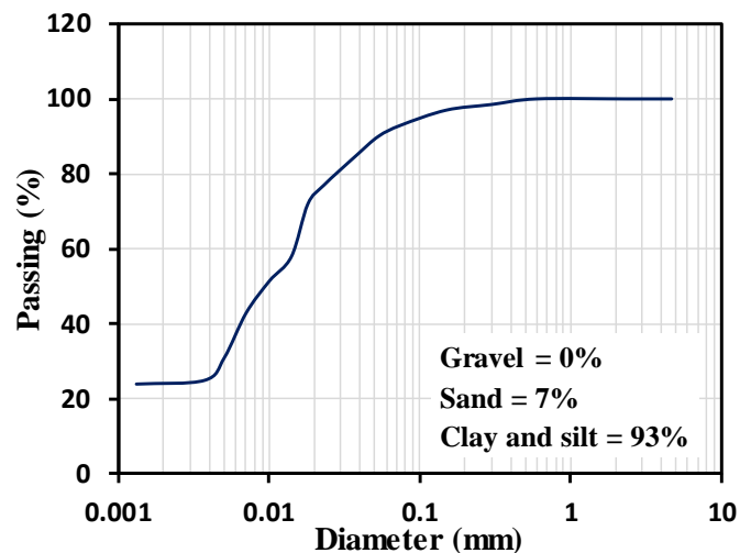
Fig. 2. Grain size distribution of landfill geomaterial.
