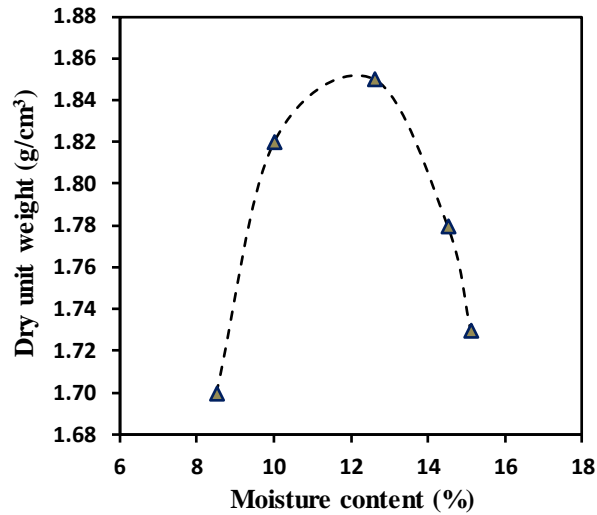
Fig. 3. Compaction curve of landfill geomaterial.
