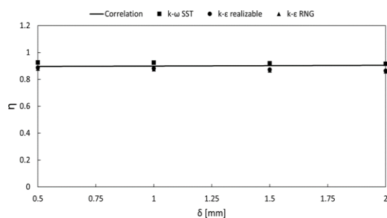
Fig. 13. Variation of the thermal performance factor with the tape thickness
